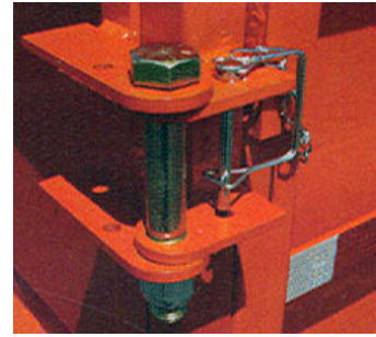
Bolted tailgate hinge & holdback pins
